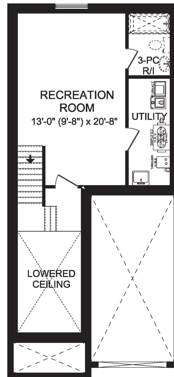
BANFF BASEMENT FLOOR PLAN OPTIONS: RECREATION ROOM
