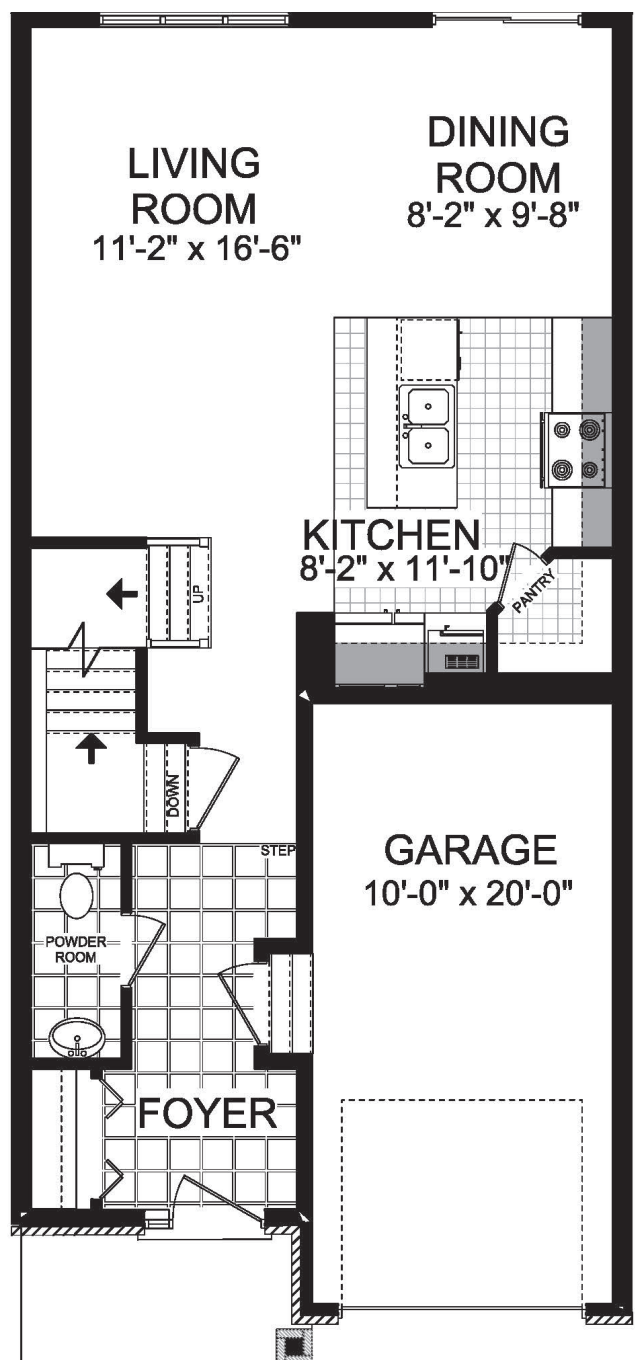
BANFF MAIN FLOOR PLAN
